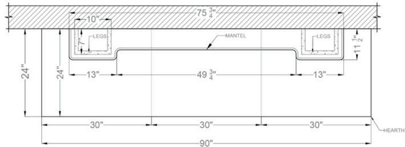
TOP VIEW
